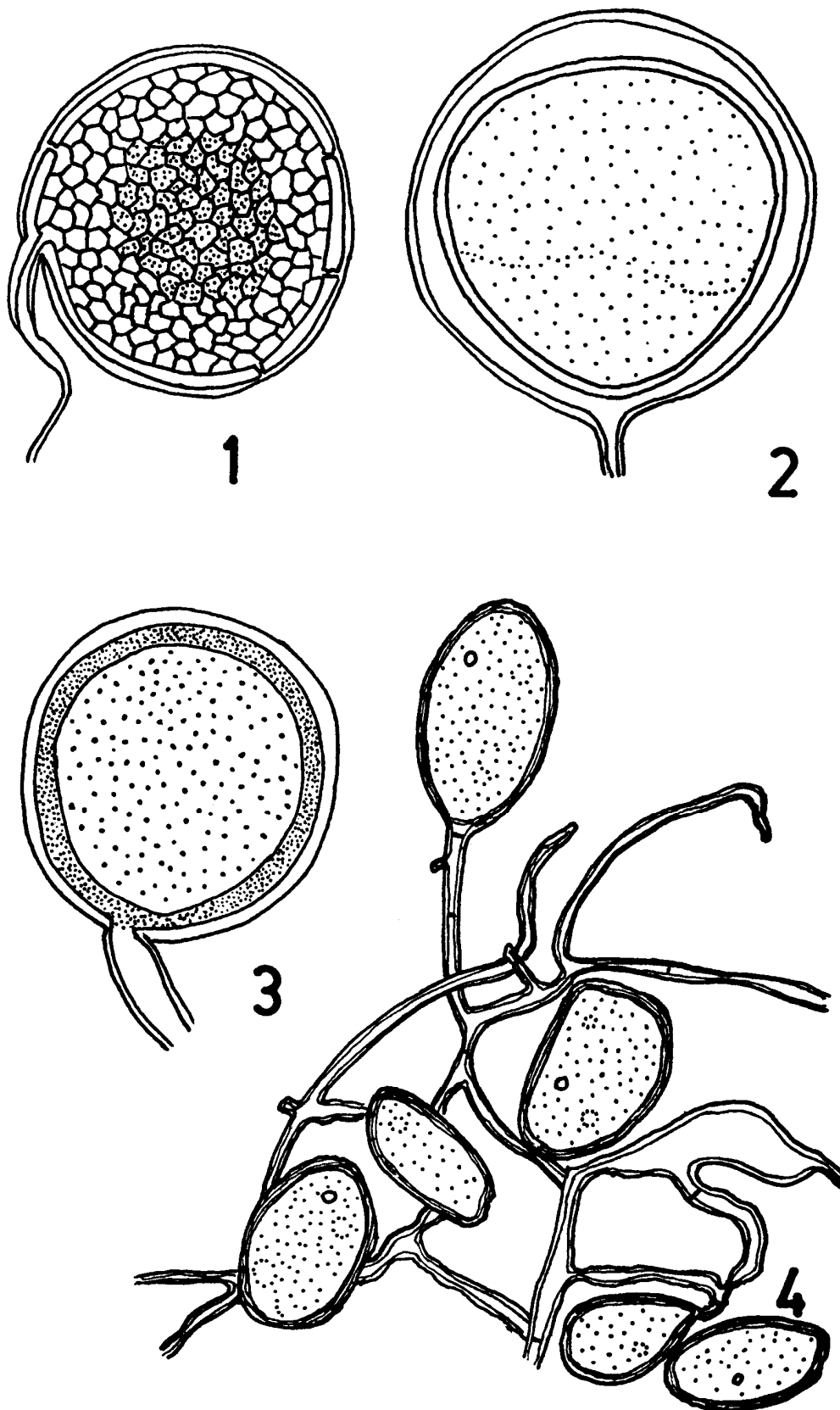
Figs. 1–4. Chlamydospores of: 1. Glomus reticulatus \times 340 . — 2. Glomus caledonius \times 420 . — 3. Glomus invermairii \times 350 . — 4. Glomus fulvus \times 40
